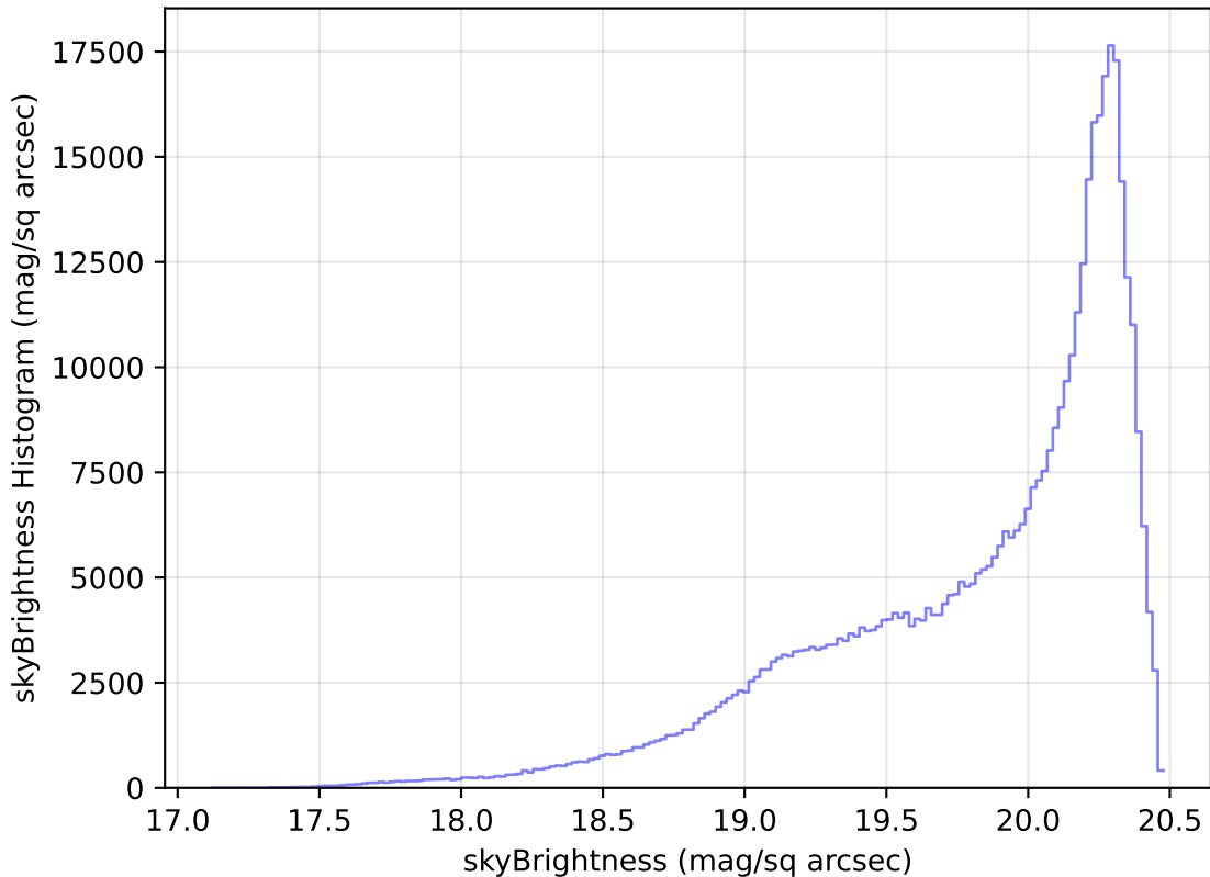
weather_cloudso30v3.4_10yrs All sky i band: skyBrightness Histogram
