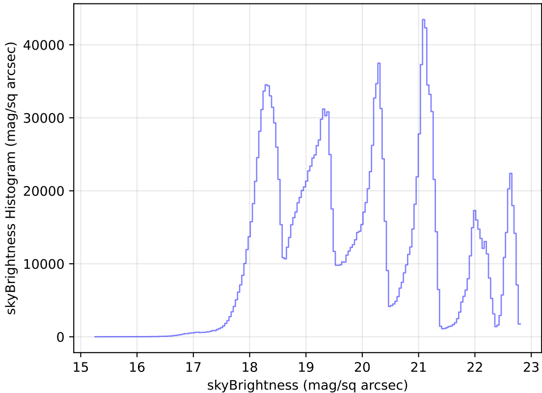
weather_cloudso30v3.4_10yrs All sky all bands: skyBrightness Histogram
