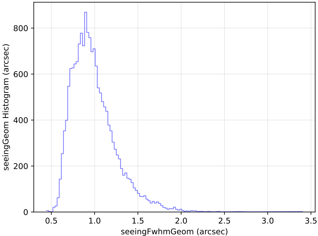
weather_cloudso30v3.4_10yrs Yr 1 u band: seeingGeom Histogram
