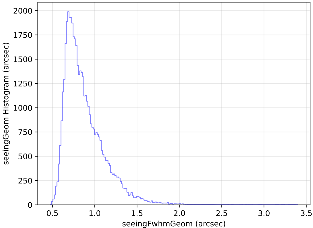
weather_cloudso30v3.4_10yrs Yr 1 r band: seeingGeom Histogram
