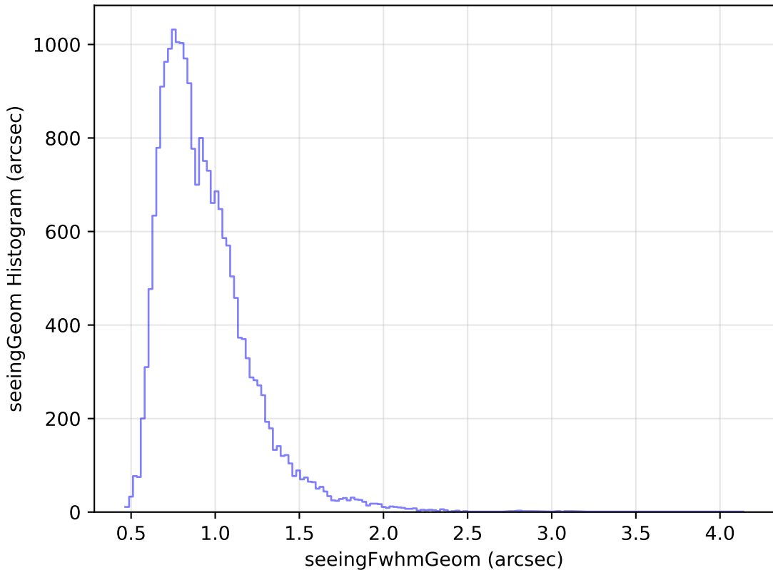
weather_cloudso30v3.4_10yrs Yr 1 g band: seeingGeom Histogram
