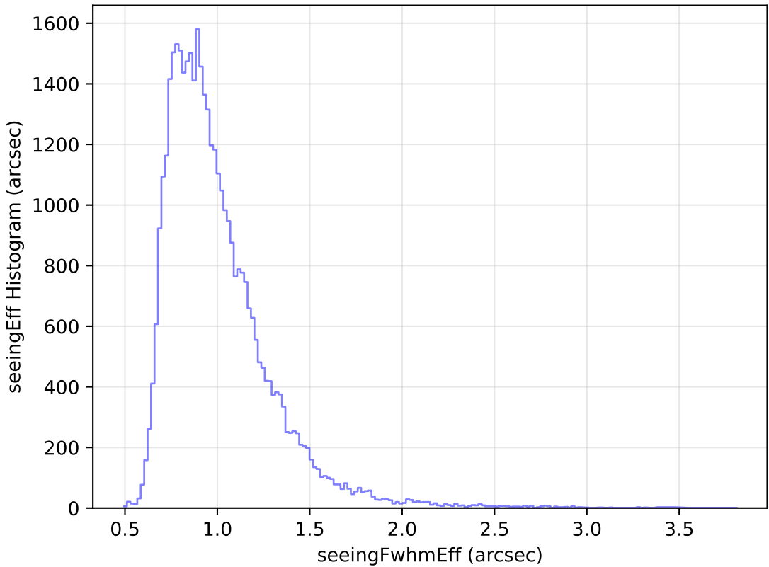
weather_cloudso30v3.4_10yrs Yr 1 z band: seeingEff Histogram
