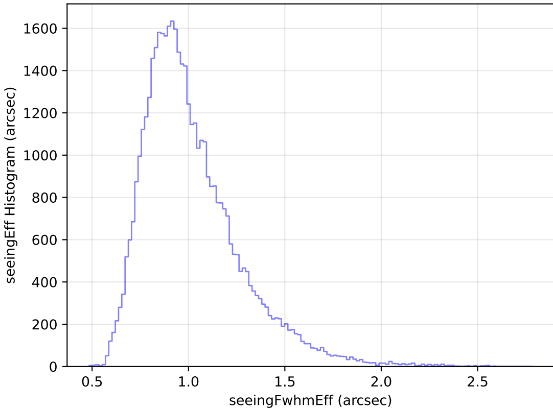
weather_cloudso30v3.4_10yrs Yr 1 y band: seeingEff Histogram
