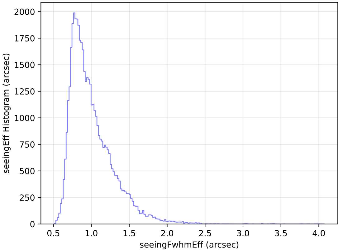
weather_cloudso30v3.4_10yrs Yr 1 r band: seeingEff Histogram
