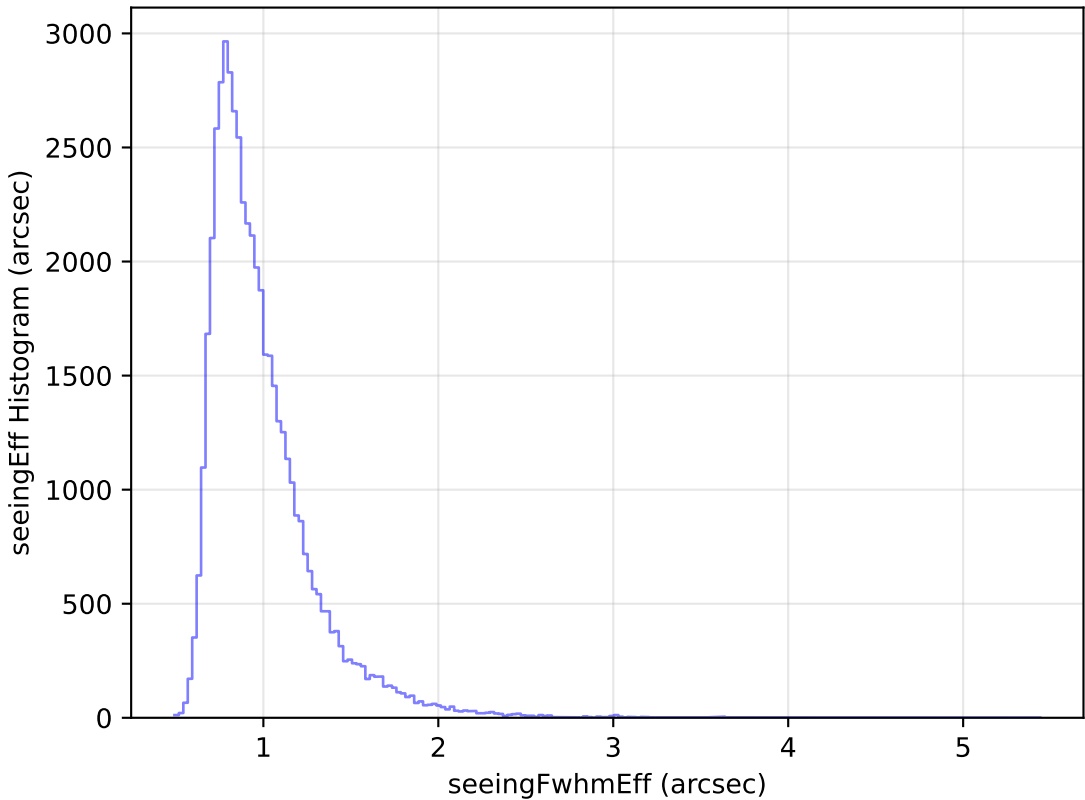
weather_cloudso30v3.4_10yrs Yr 1 i band: seeingEff Histogram
