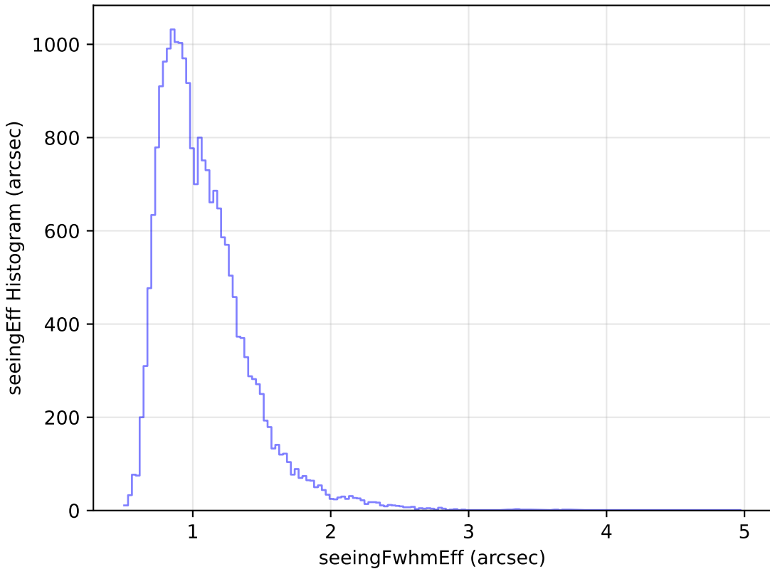
weather_cloudso30v3.4_10yrs Yr 1 g band: seeingEff Histogram
