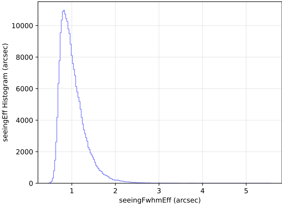
weather_cloudso30v3.4_10yrs Yr 1 all bands: seeingEff Histogram
