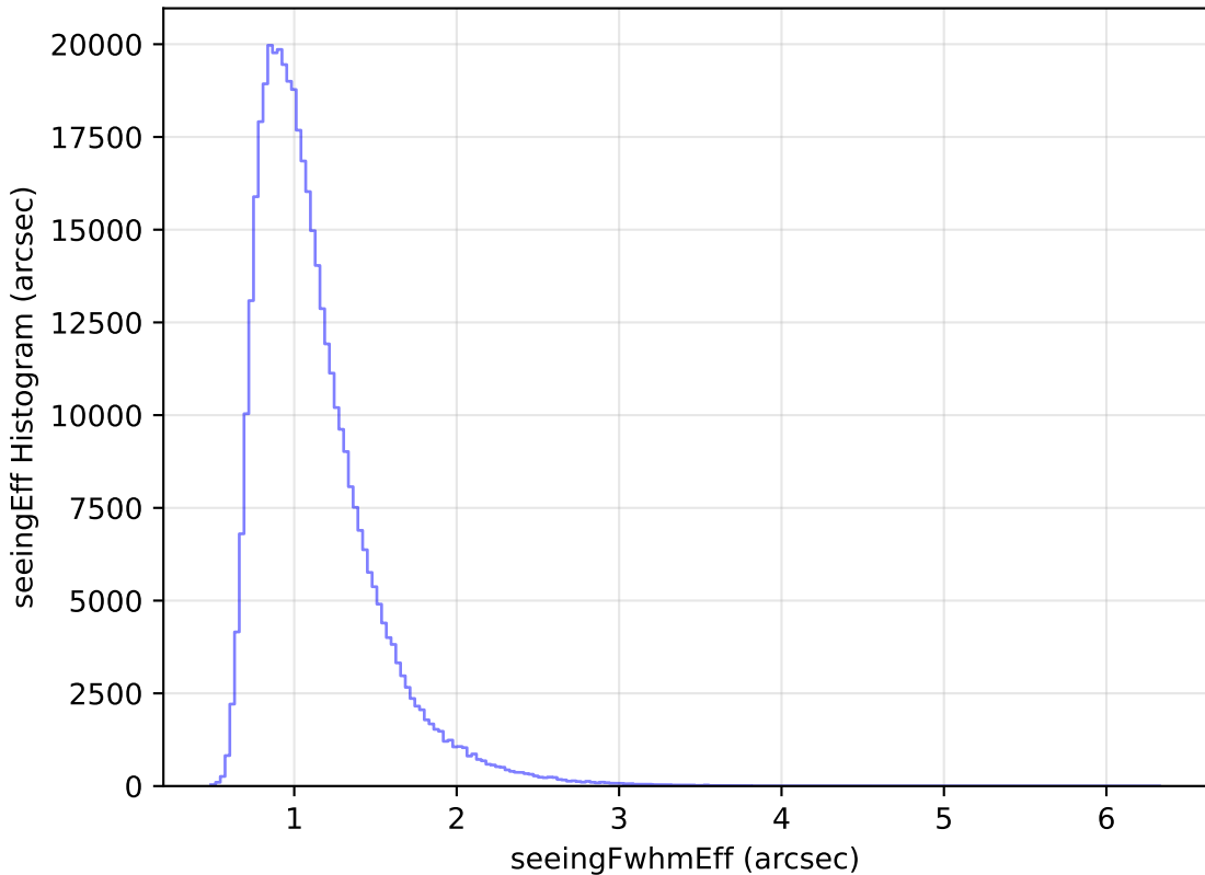
weather_cloudso30v3.4_10yrs WFD z band: seeingEff Histogram
