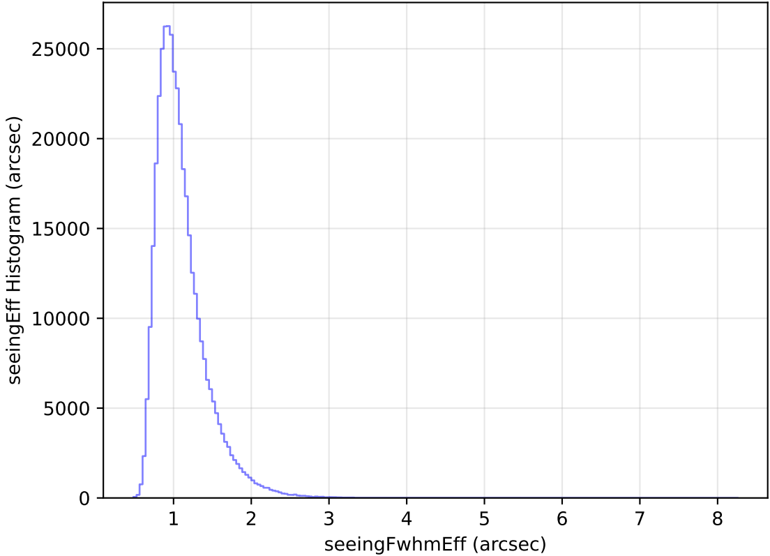
weather_cloudso30v3.4_10yrs WFD y band: seeingEff Histogram
