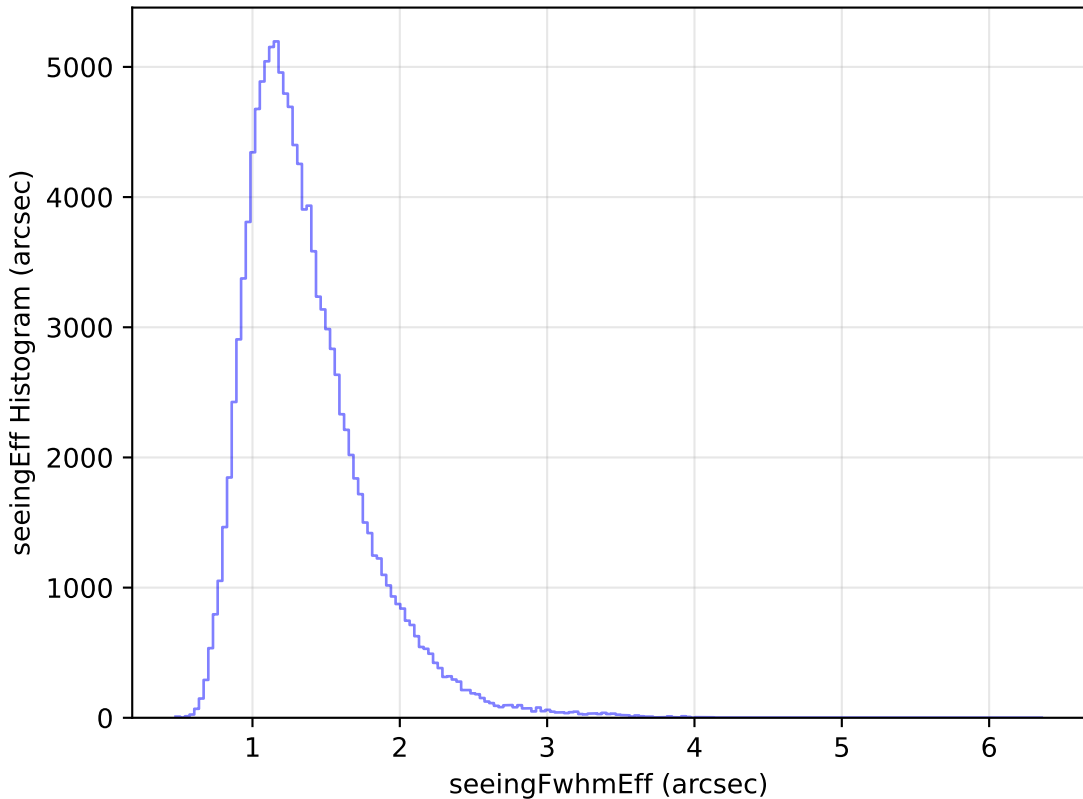
weather_cloudso30v3.4_10yrs WFD u band: seeingEff Histogram
