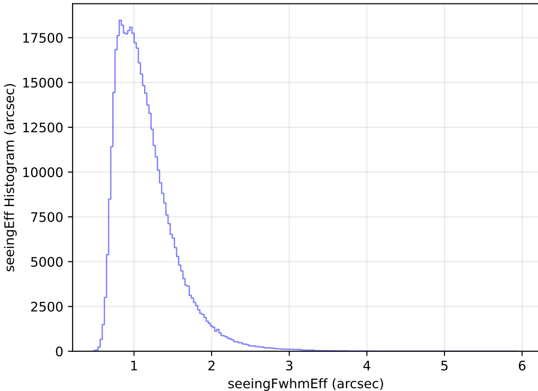
weather_cloudso30v3.4_10yrs WFD r band: seeingEff Histogram
