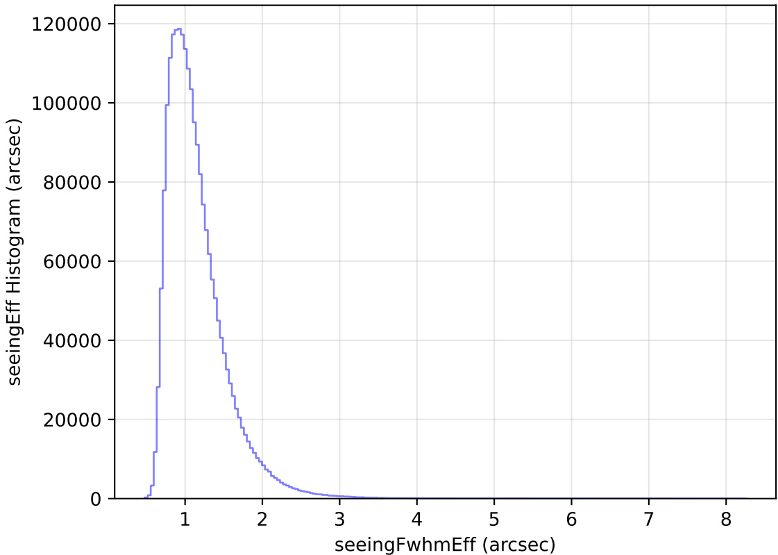
weather_cloudso30v3.4_10yrs WFD all bands: seeingEff Histogram
