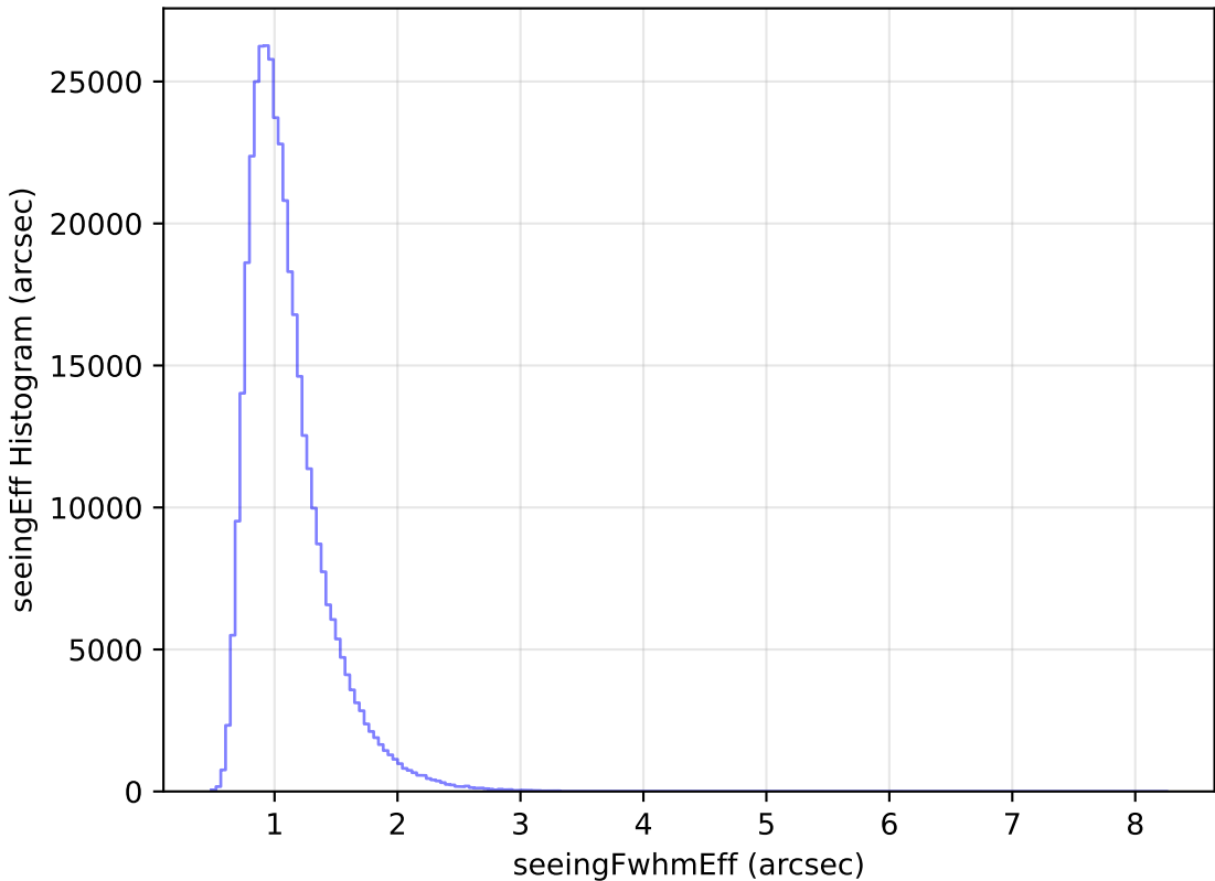
weather_cloudso30v3.4_10yrs All sky y band: seeingEff Histogram
