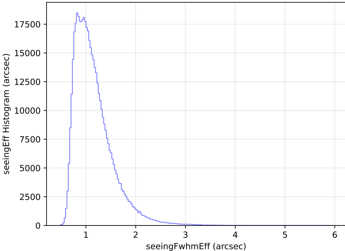
weather_cloudso30v3.4_10yrs All sky r band: seeingEff Histogram
