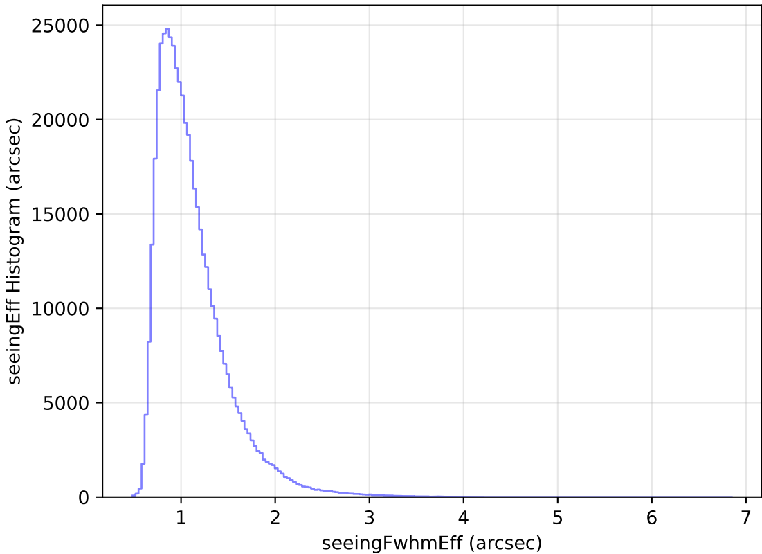
weather_cloudso30v3.4_10yrs All sky i band: seeingEff Histogram
