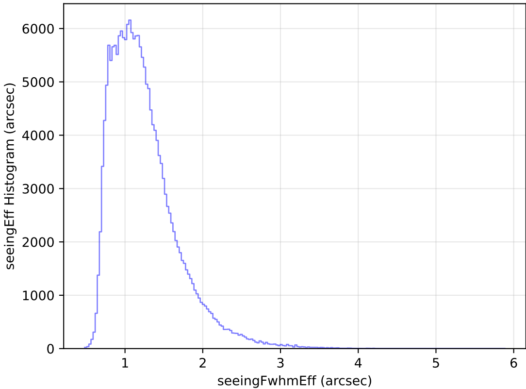
weather_cloudso30v3.4_10yrs All sky g band: seeingEff Histogram
