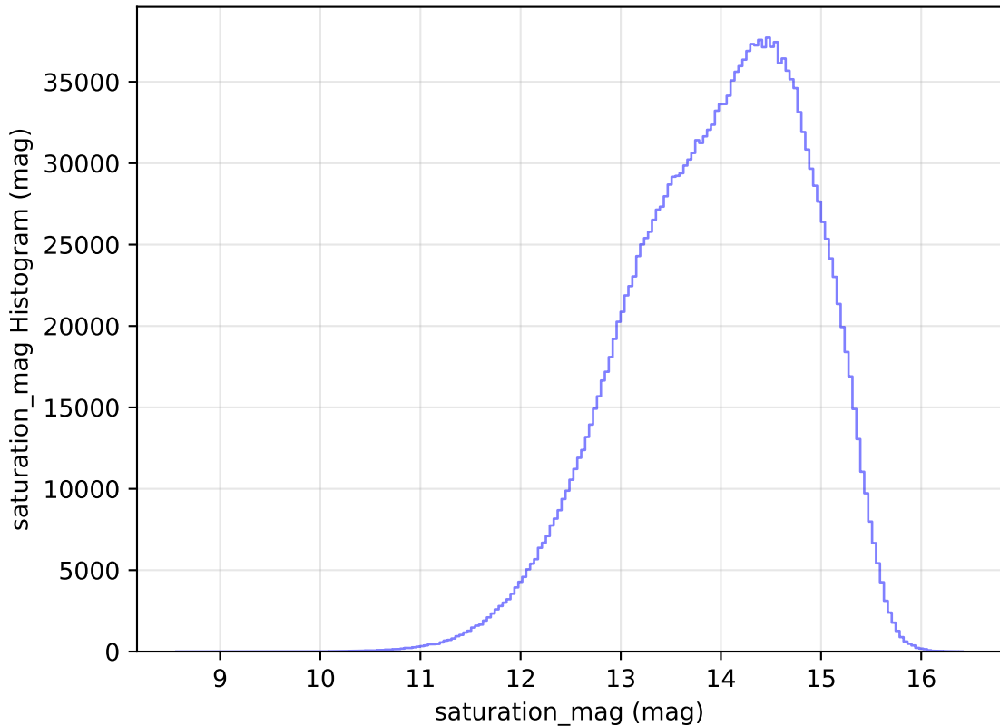
weather_cloudso30v3.4_10yrs WFD all bands: saturation_mag Histogram
