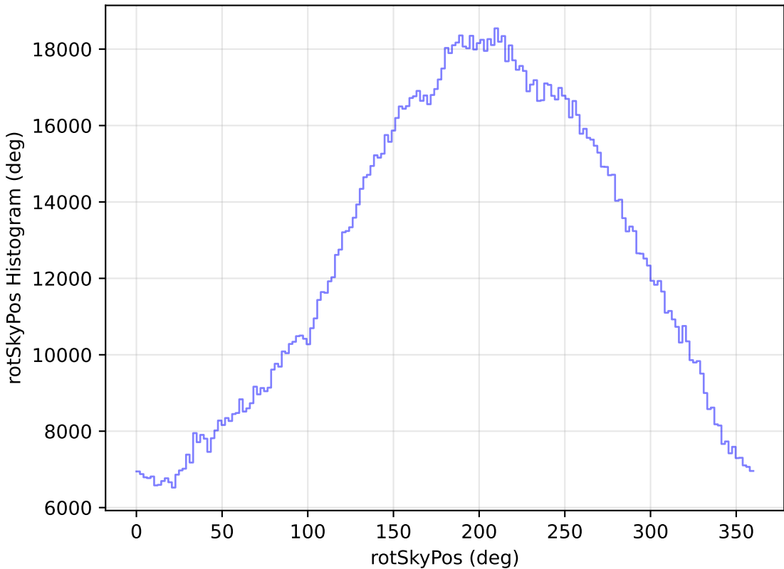
weather_cloudso30v3.4_10yrs WFD all bands: rotSkyPos Histogram
