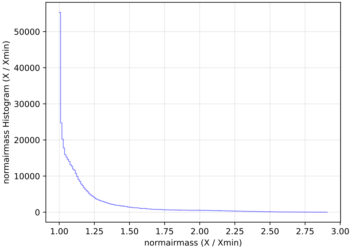
weather_cloudso30v3.4_10yrs WFD z band: normairmass Histogram
