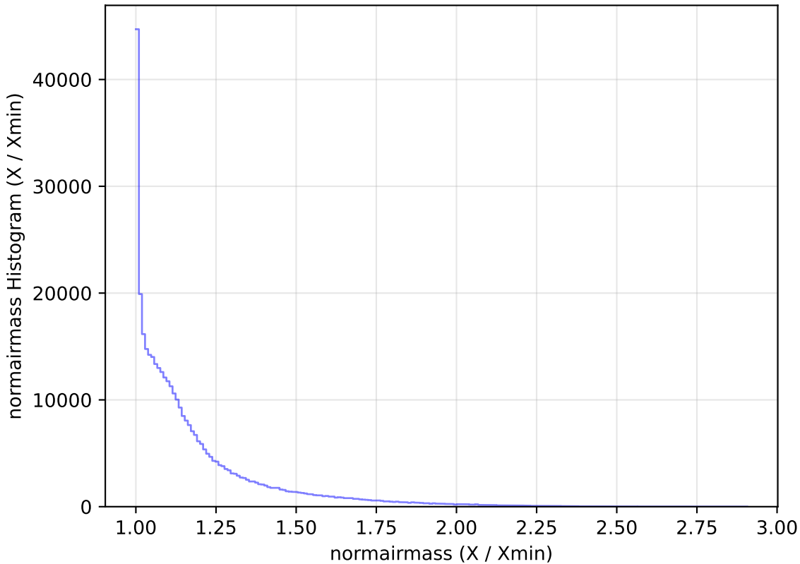
weather_cloudso30v3.4_10yrs WFD y band: normairmass Histogram
