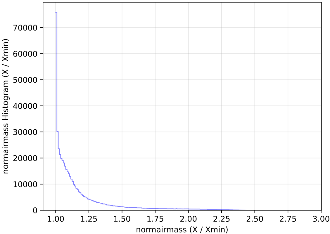
weather_cloudso30v3.4_10yrs WFD r band: normairmass Histogram
