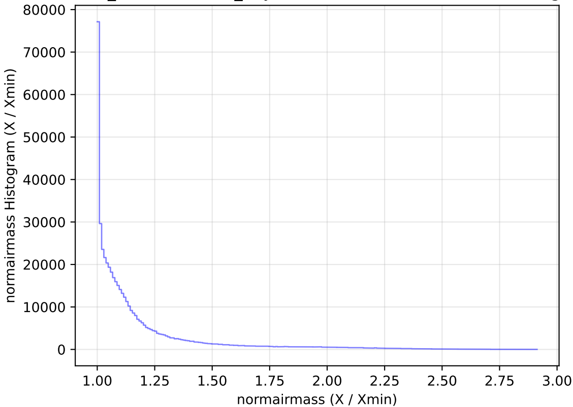
weather_cloudso30v3.4_10yrs WFD i band: normairmass Histogram
