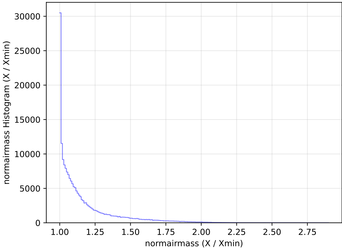
weather_cloudso30v3.4_10yrs WFD g band: normairmass Histogram
