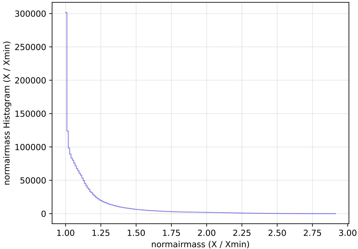
weather_cloudso30v3.4_10yrs WFD all bands: normairmass Histogram
