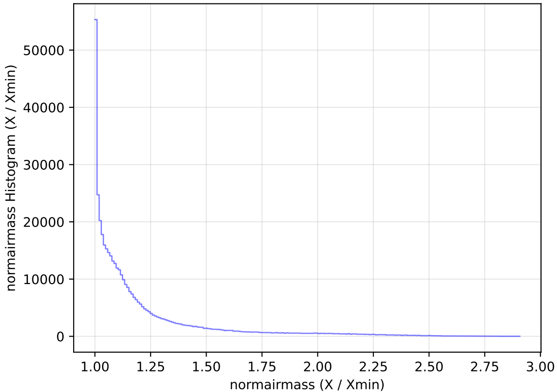
weather_cloudso30v3.4_10yrs All sky z band: normairmass Histogram
