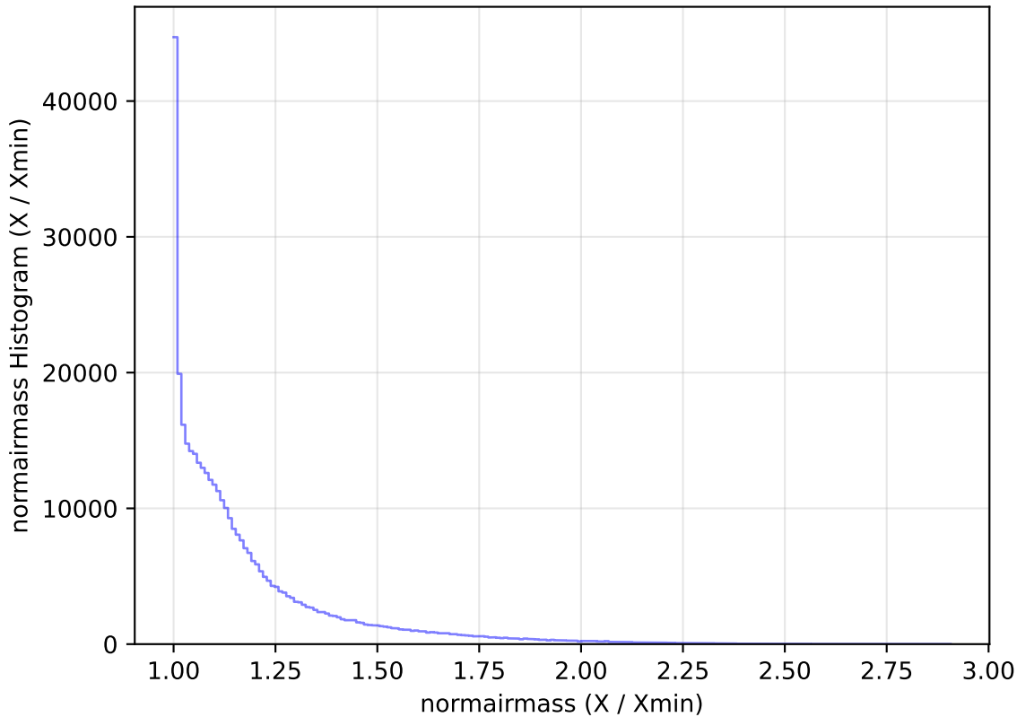
weather_cloudso30v3.4_10yrs All sky y band: normairmass Histogram
