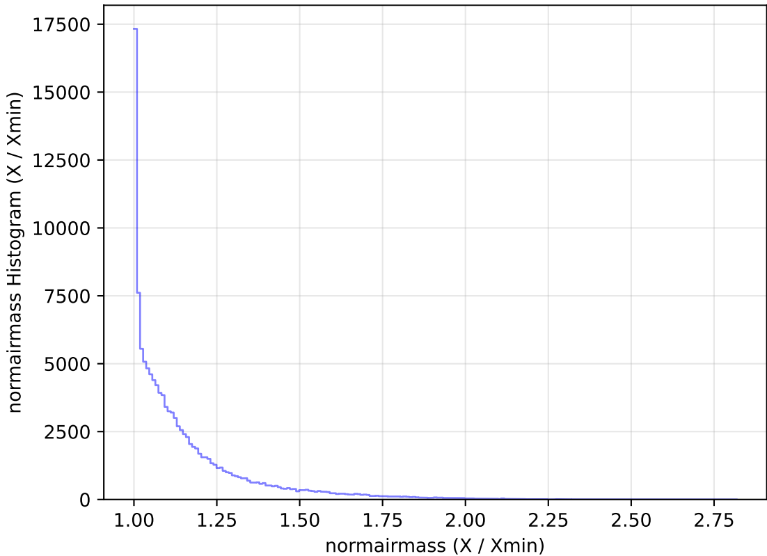
weather_cloudso30v3.4_10yrs All sky u band: normairmass Histogram
