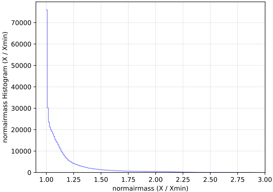
weather_cloudso30v3.4_10yrs All sky r band: normairmass Histogram
