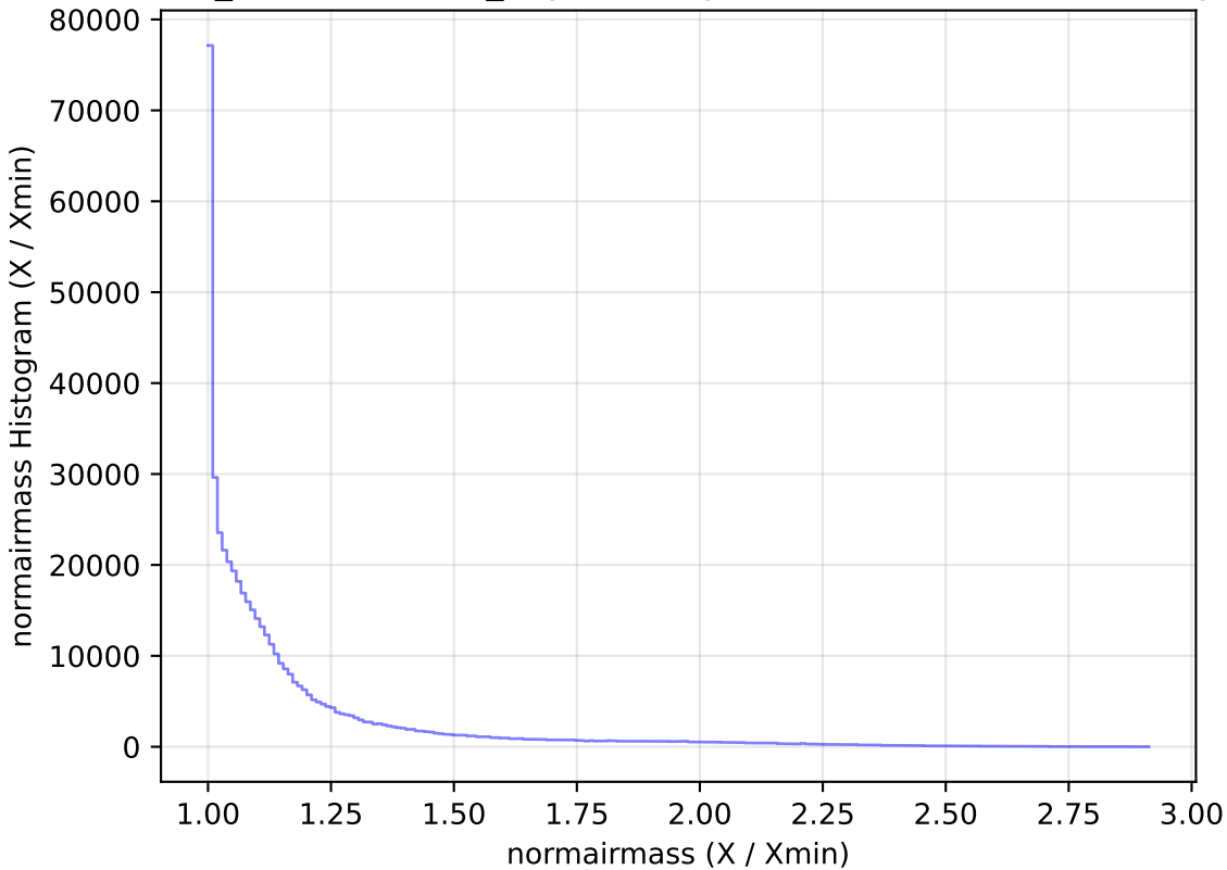
weather_cloudso30v3.4_10yrs All sky i band: normairmass Histogram
