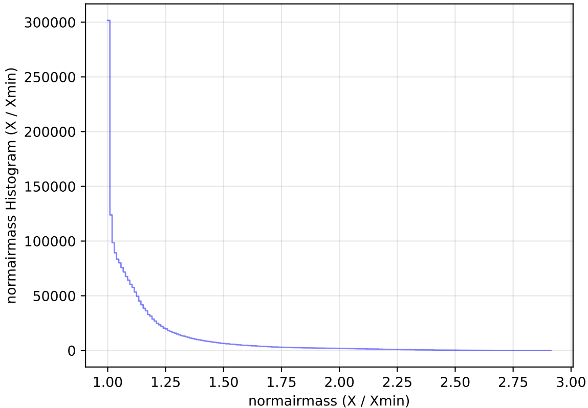
weather_cloudso30v3.4_10yrs All sky all bands: normairmass Histogram
