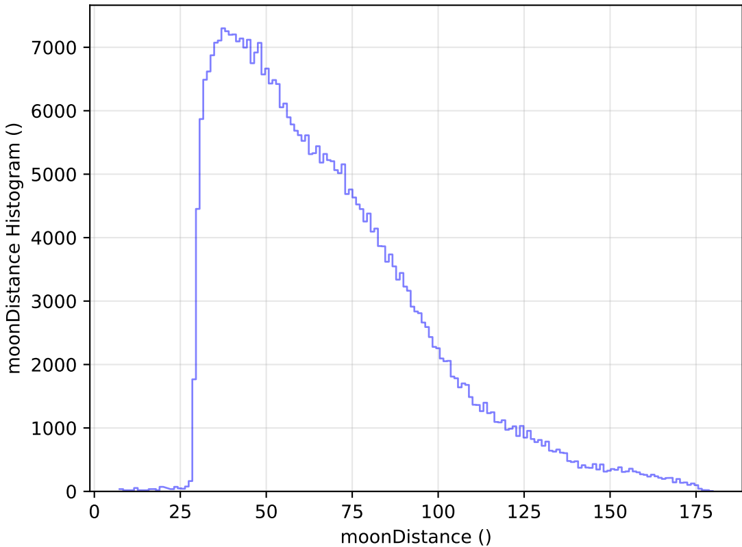
weather_cloudso30v3.4_10yrs WFD y band: moonDistance Histogram
