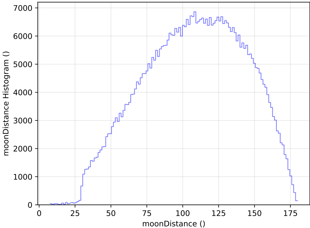
weather_cloudso30v3.4_10yrs WFD r band: moonDistance Histogram
