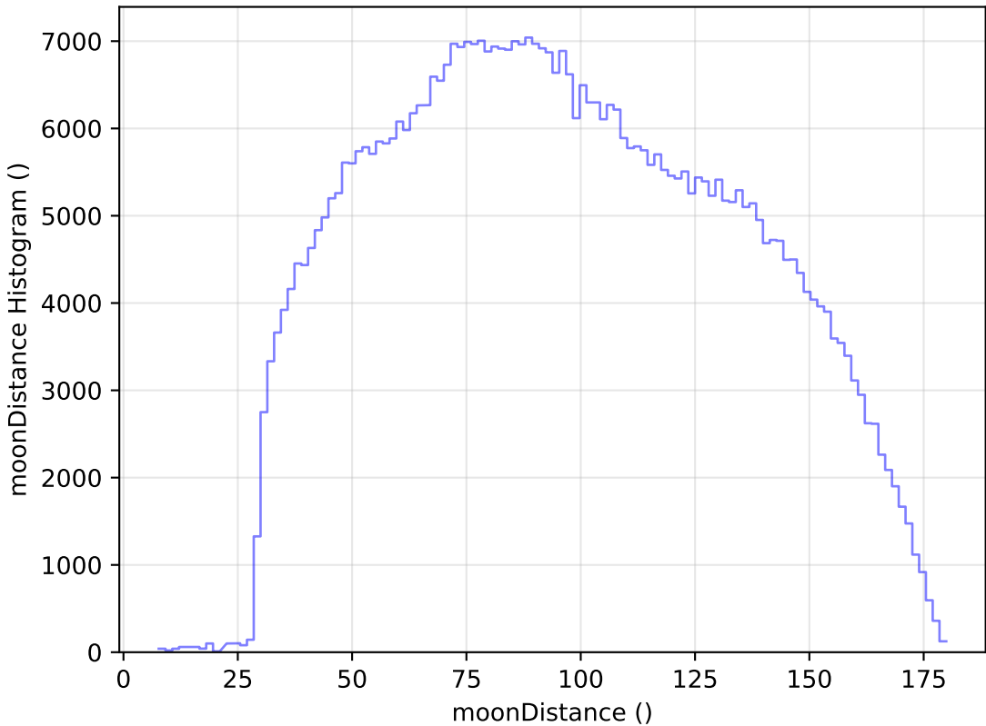
weather_cloudso30v3.4_10yrs WFD i band: moonDistance Histogram
