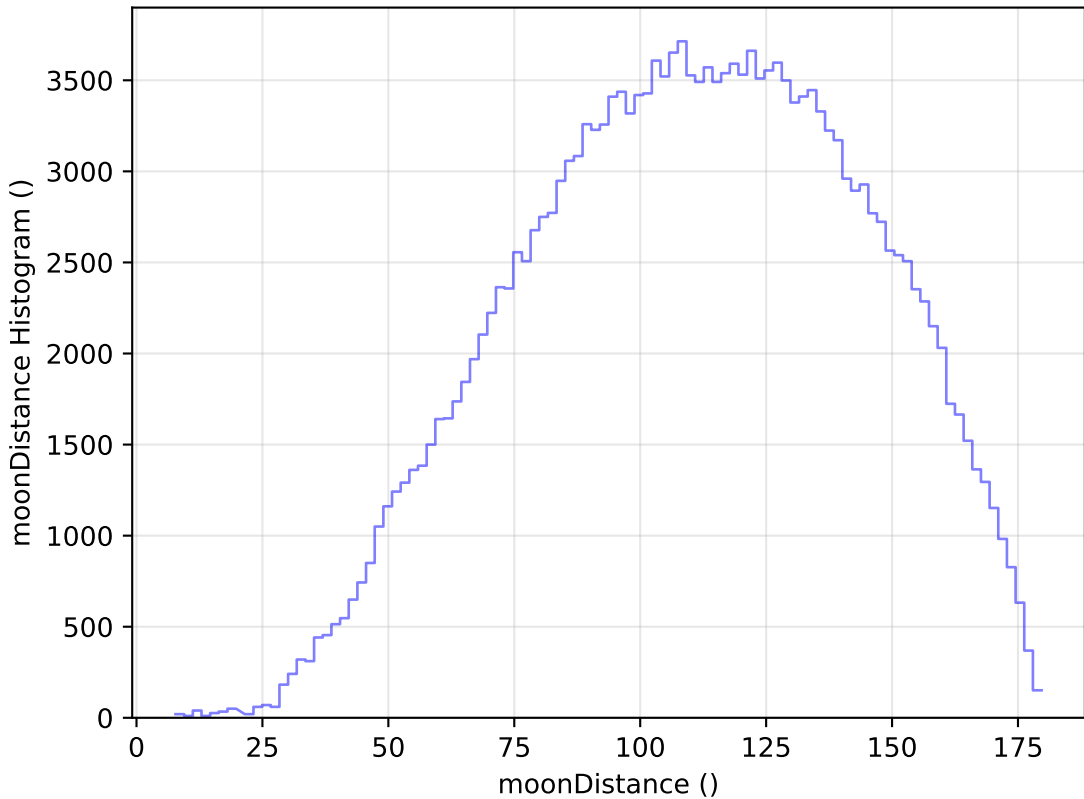
weather_cloudso30v3.4_10yrs WFD g band: moonDistance Histogram
