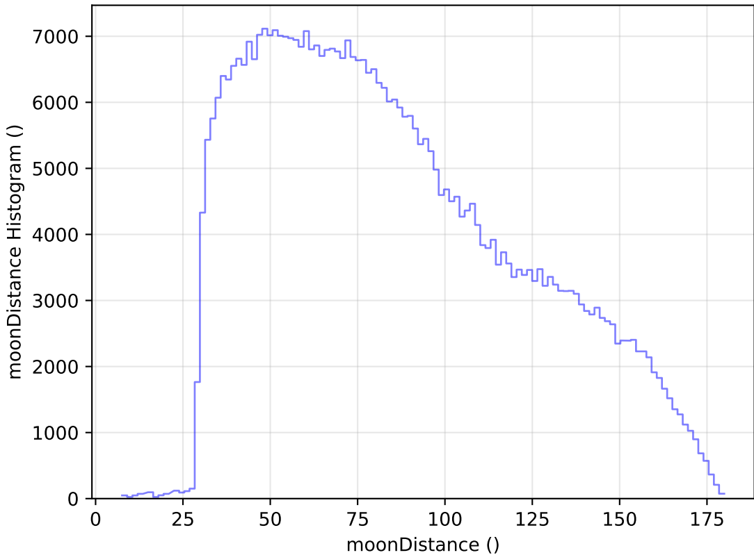
weather_cloudso30v3.4_10yrs All sky z band: moonDistance Histogram
