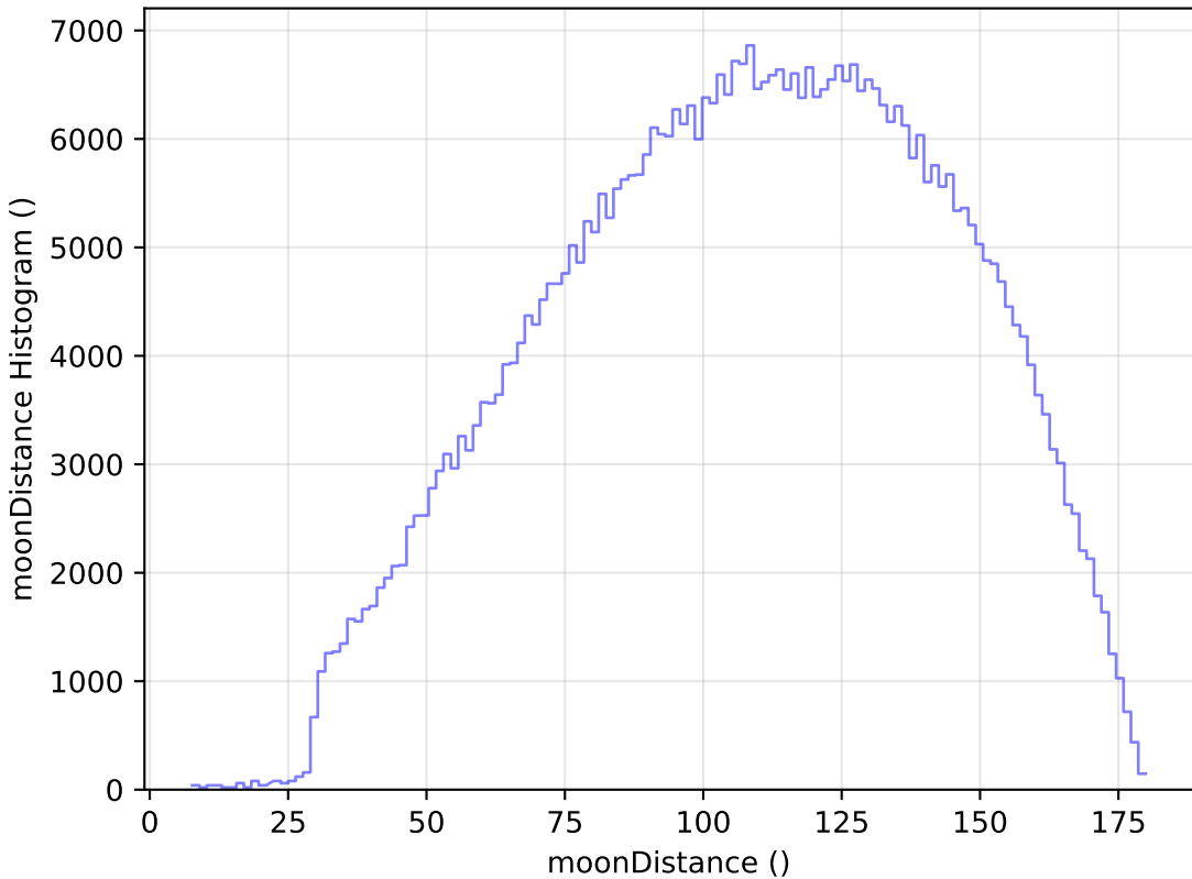
weather_cloudso30v3.4_10yrs All sky r band: moonDistance Histogram
