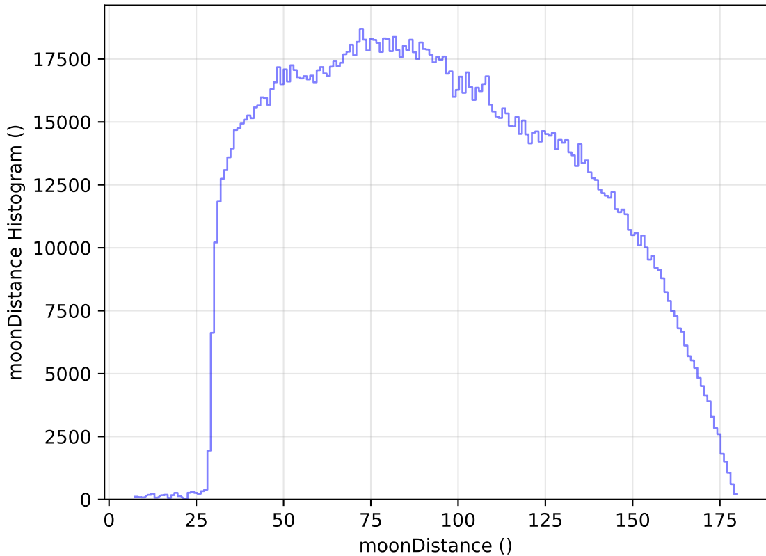
weather_cloudso30v3.4_10yrs All sky all bands: moonDistance Histogram
