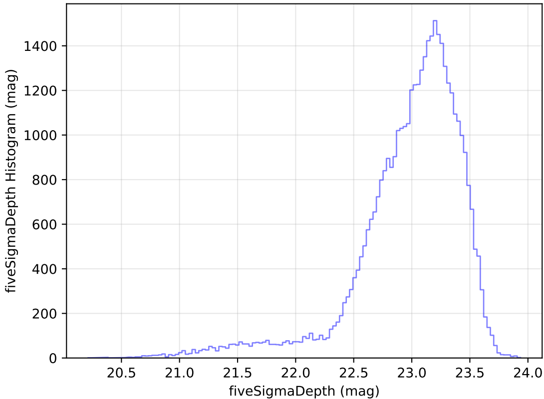
weather_cloudso30v3.4_10yrs Yr 1 z band: fiveSigmaDepth Histogram
