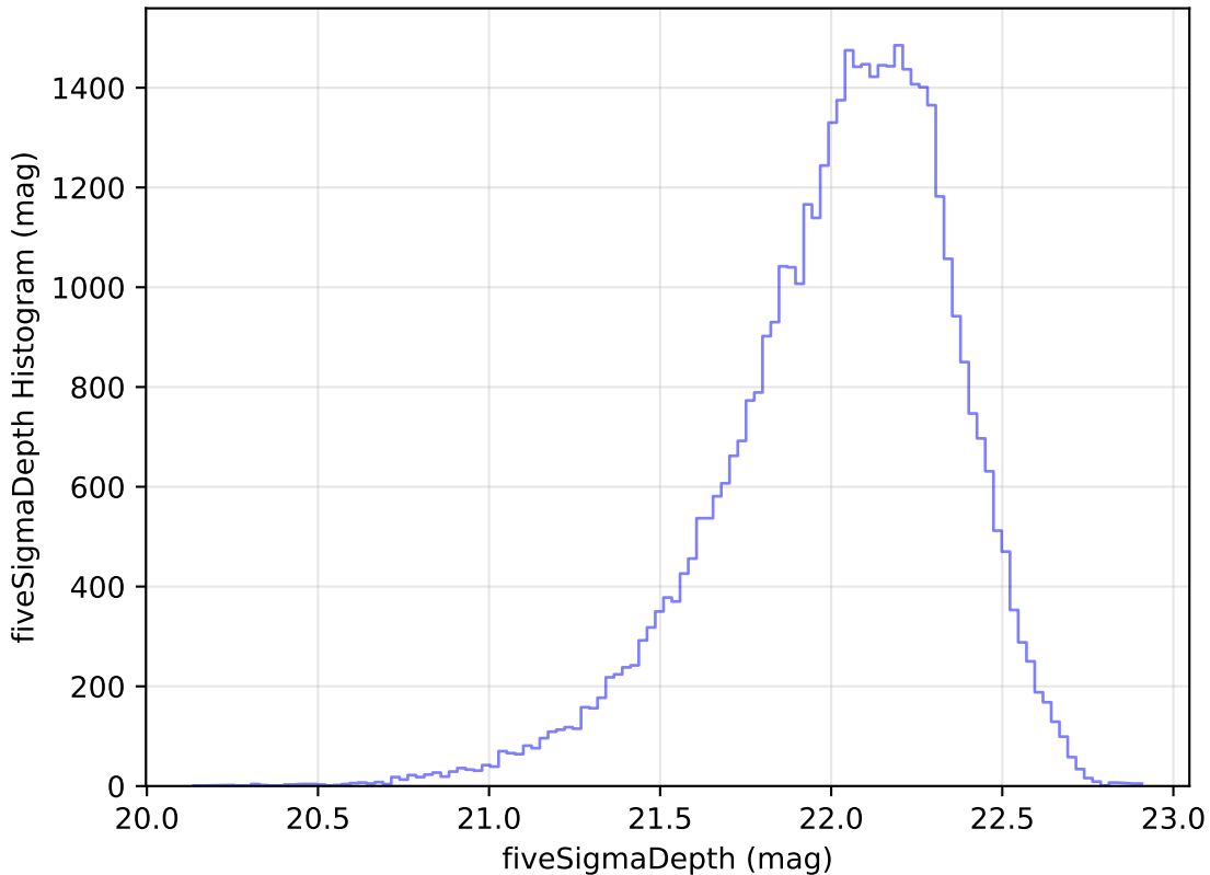
weather_cloudso30v3.4_10yrs Yr 1 y band: fiveSigmaDepth Histogram
