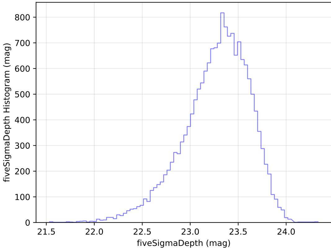
weather_cloudso30v3.4_10yrs Yr 1 u band: fiveSigmaDepth Histogram
