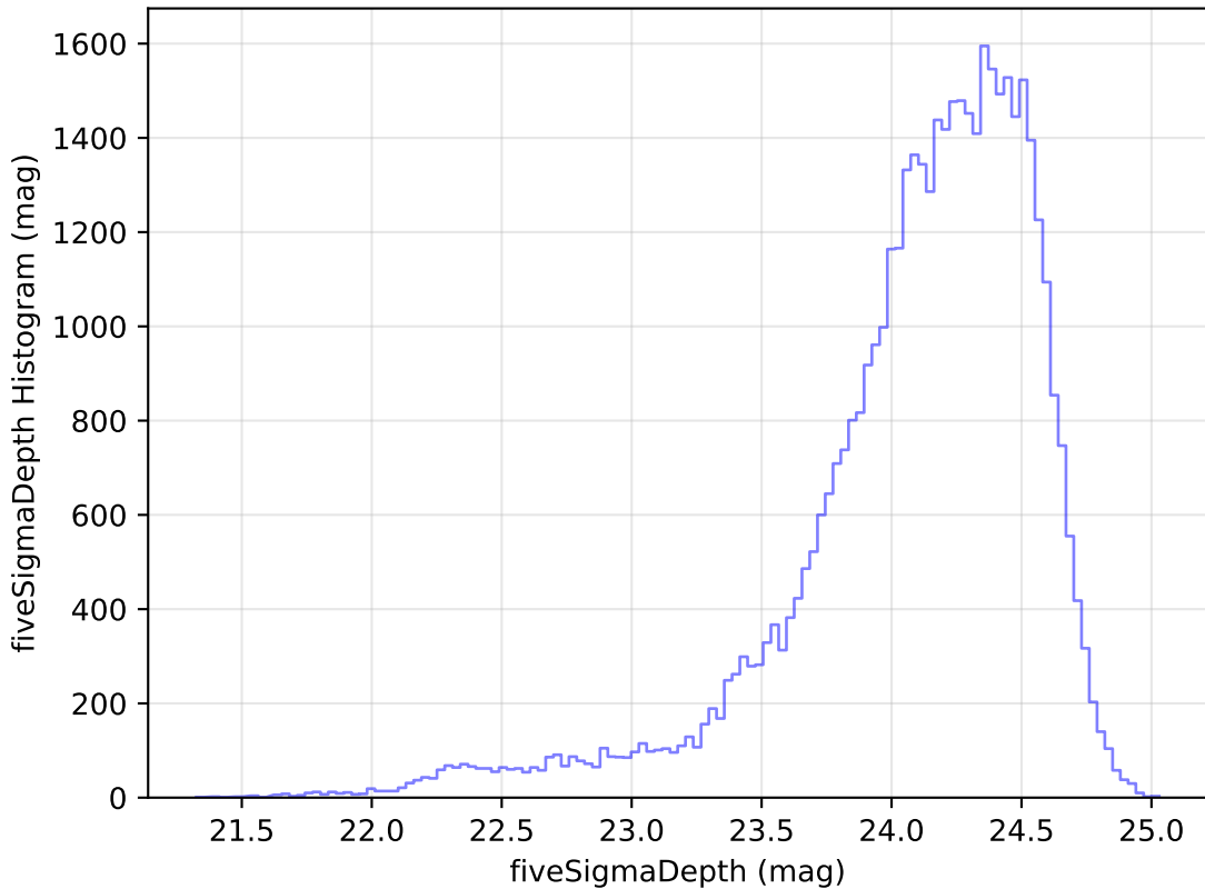
weather_cloudso30v3.4_10yrs Yr 1 r band: fiveSigmaDepth Histogram
