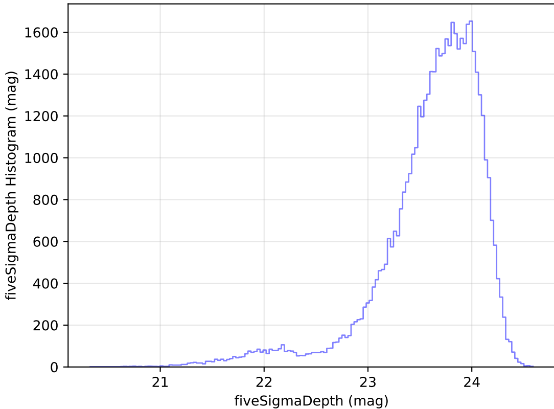
weather_cloudso30v3.4_10yrs Yr 1 i band: fiveSigmaDepth Histogram
