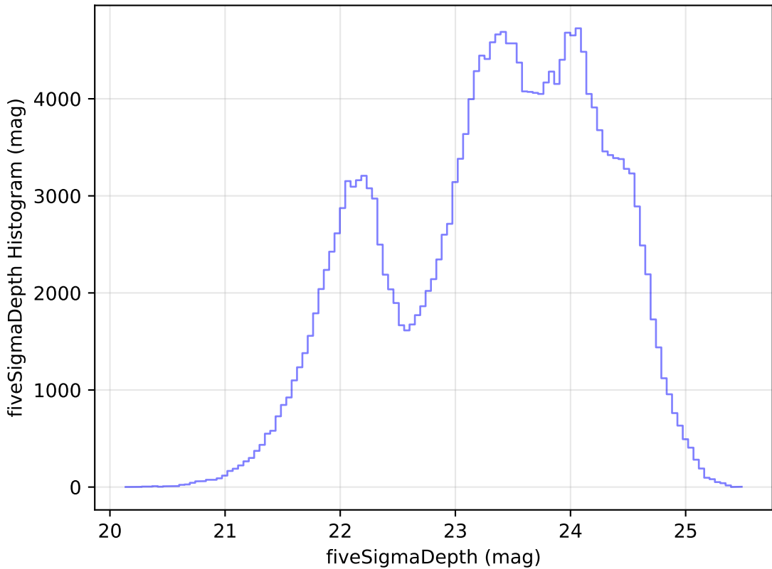
weather_cloudso30v3.4_10yrs Yr 1 all bands: fiveSigmaDepth Histogram
