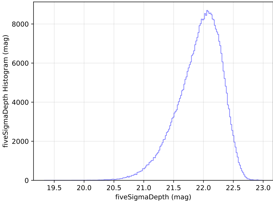
weather_cloudso30v3.4_10yrs WFD y band: fiveSigmaDepth Histogram
