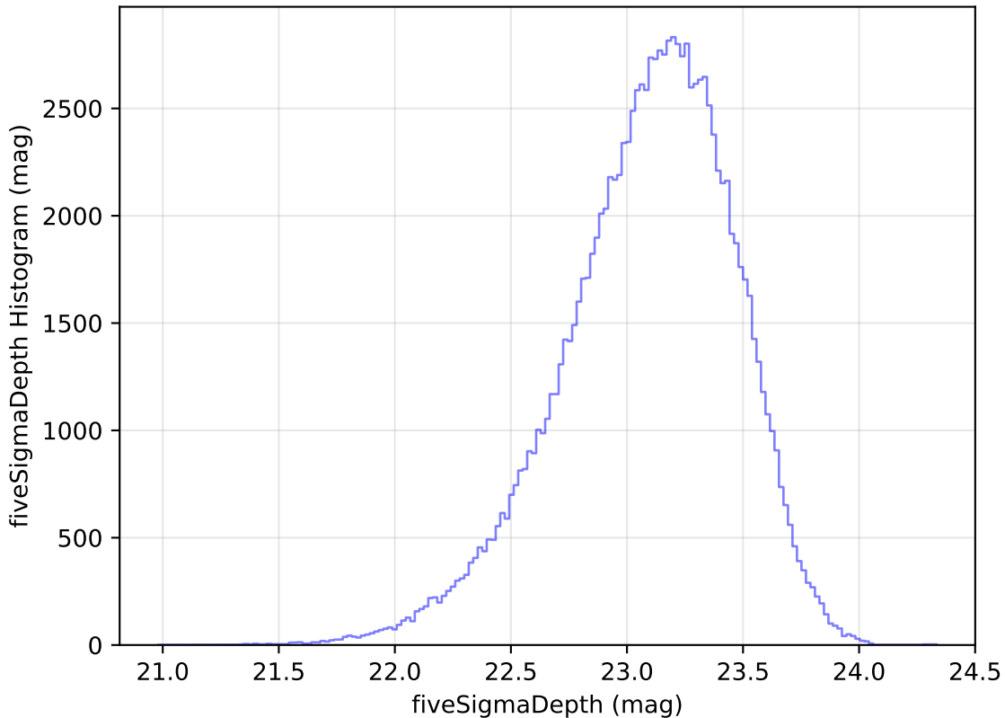
weather_cloudso30v3.4_10yrs WFD u band: fiveSigmaDepth Histogram
