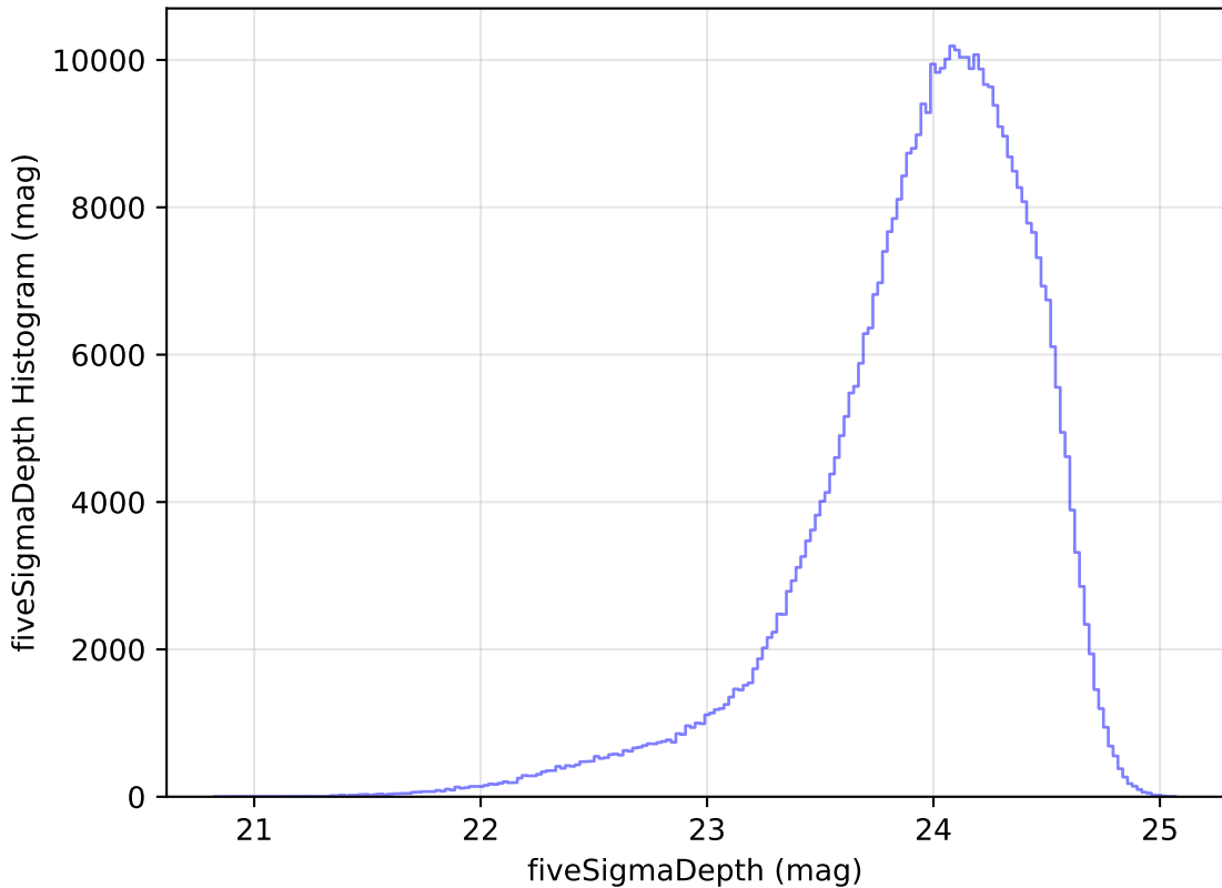
weather_cloudso30v3.4_10yrs WFD r band: fiveSigmaDepth Histogram
